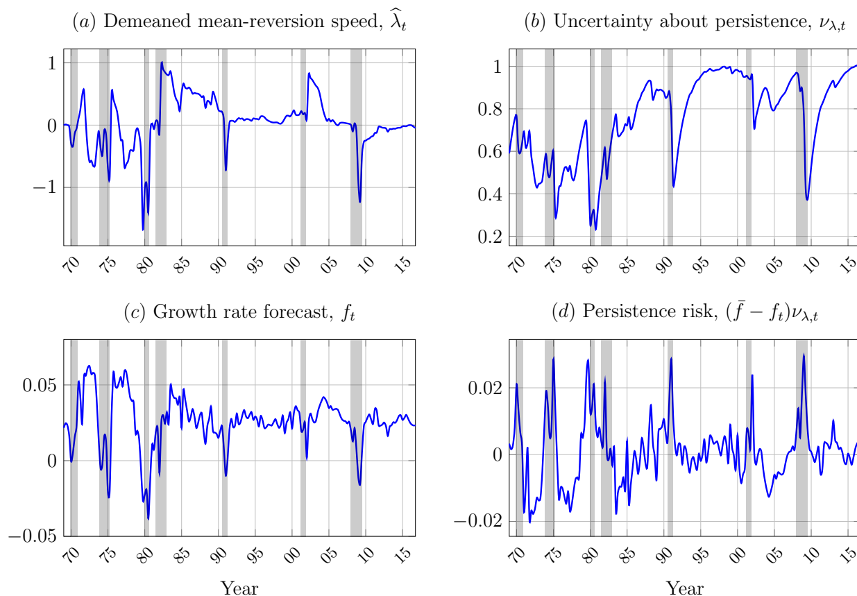
Figure 1: Historical paths of the state variables.
